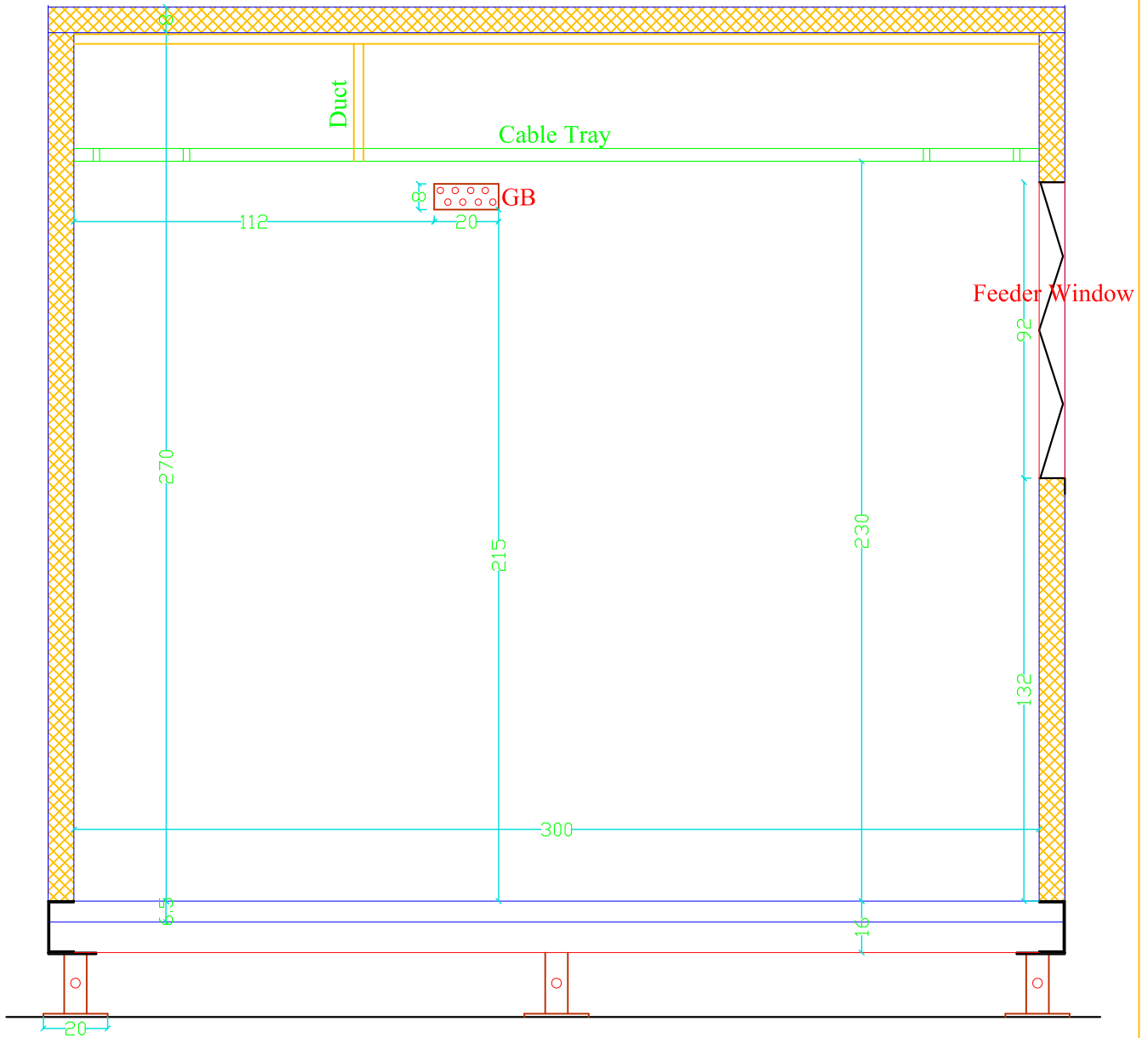
View A
