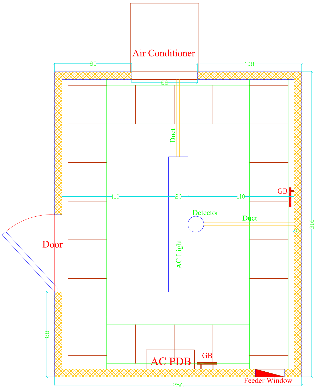
PLAN
